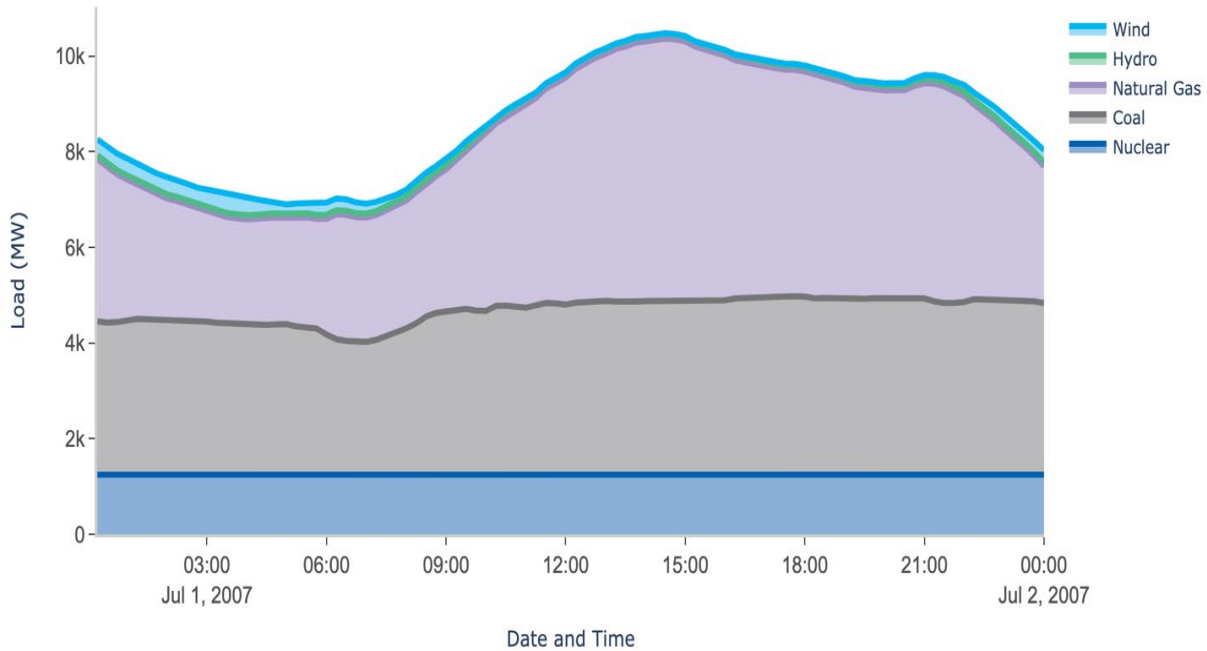
Figure 1. ERCOT generation by fuel source July 1, 2007 Source: (ERCOT 2020)
